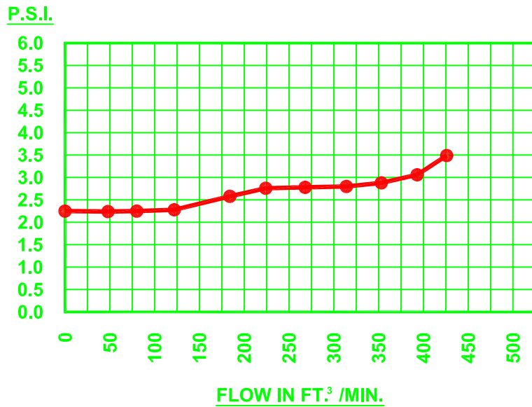
Curve for PRESSURE side of 2.5" Equate PV Valve - 2.2 PSI data based on air flow
