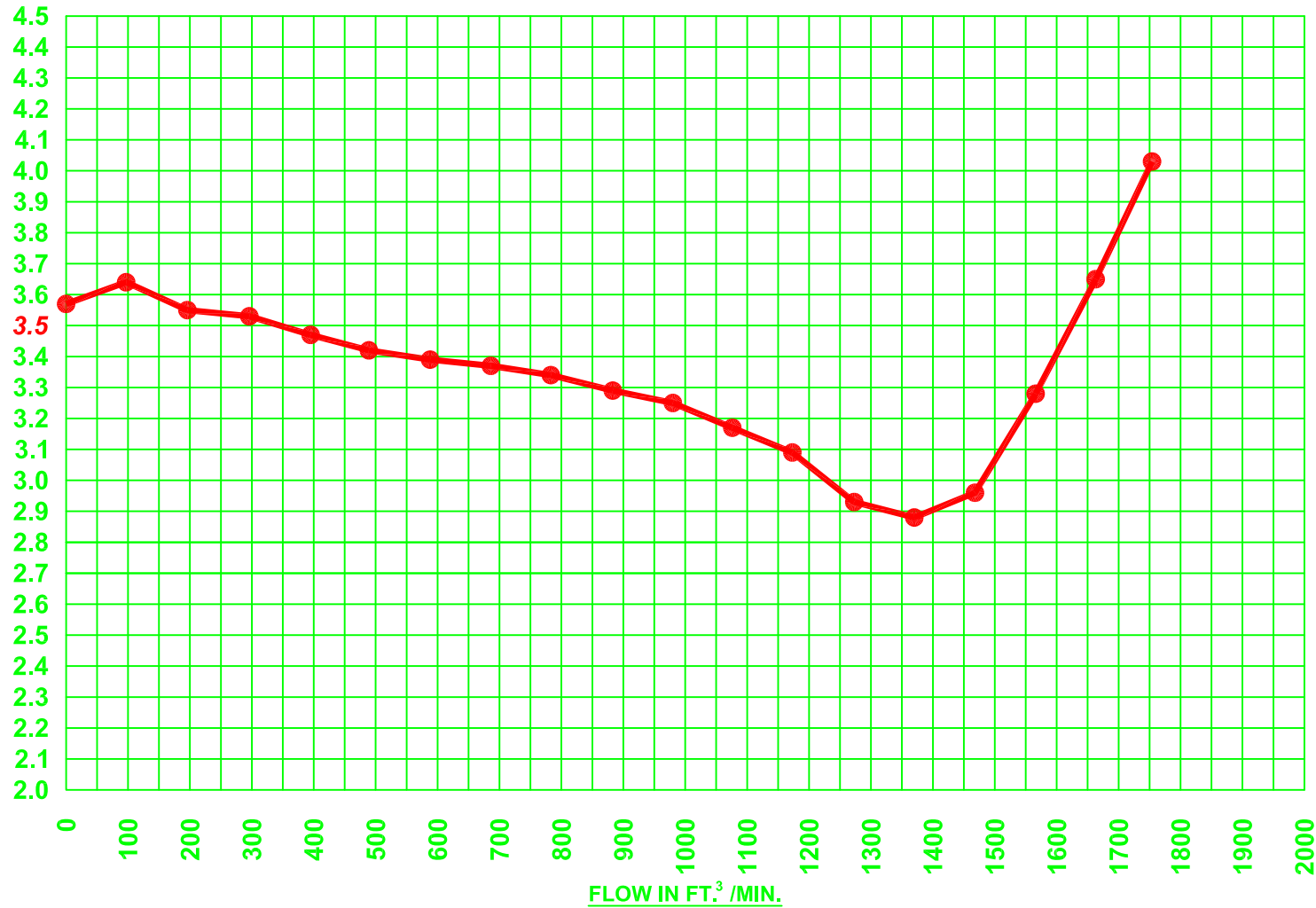
CURVE FOR PRESSURE SIDE OF 6" PV VALVE - 3.5 PSI
