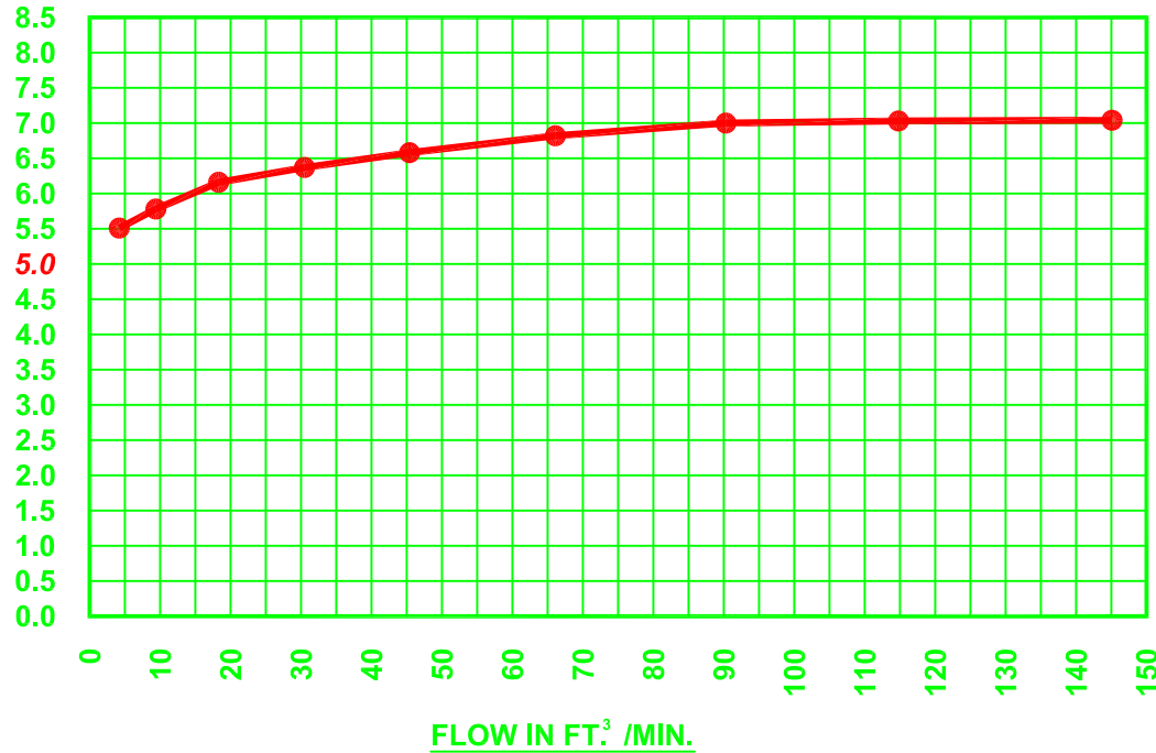
Curve for PRESSURE side of 4" Equate PV Valve - 5.0 PSI
