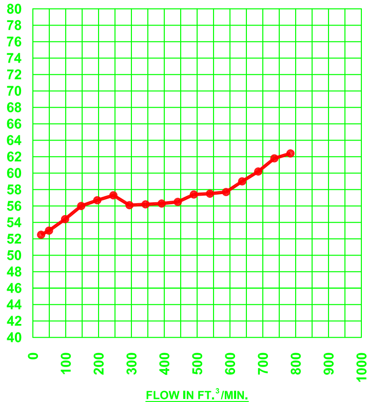
Curve for Vacuum Side of SUPERAC 6" PV Valve - 2.0 PSI data based on air flow
